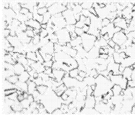
FIG. 2 Apparent Grain Size of Tungsten Carbide plus 10 % Cobalt (1500×)
