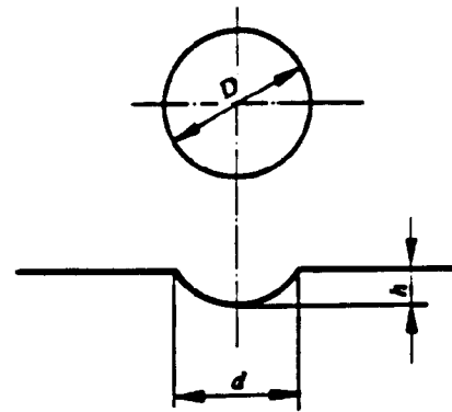
FIG. 2 Principle of Test
