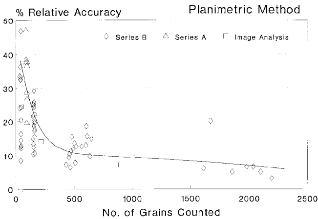
NOTE 1—The image analysis results for the same micrographs. FIG. X1.3 Relationship Between the Number of Grains Counted and the Percent Relative Accuracy for the Planimetric Method
