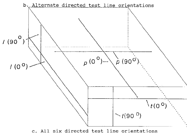
FIG. 7 Schematic Showing the Six Possible Directed Test Line Orientations for Grain Size Measurement
